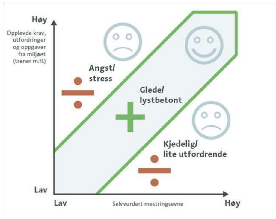
Figur 3: Flytsonmodellen
